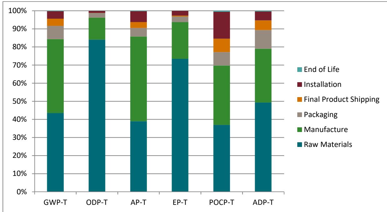
Figure 3: VDS Lite by Forster Framing System Environmental Impact Potentials (TRACI 2.1)
