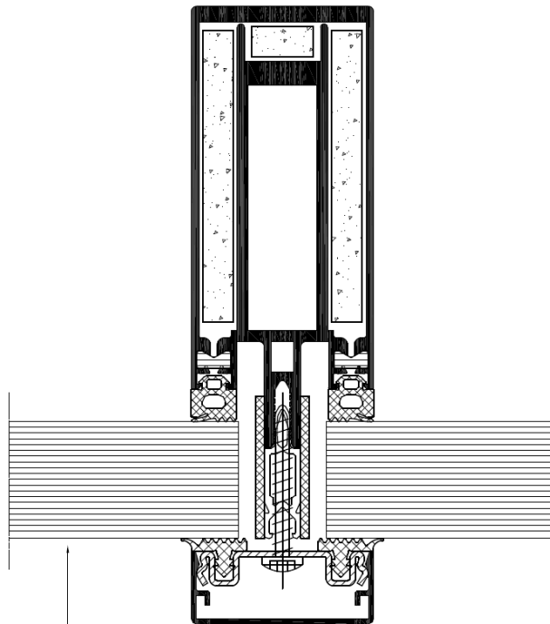
① CONTRAFLAM 30 (16 mm thick minimum) (edge-cover 13 mm minimum)
