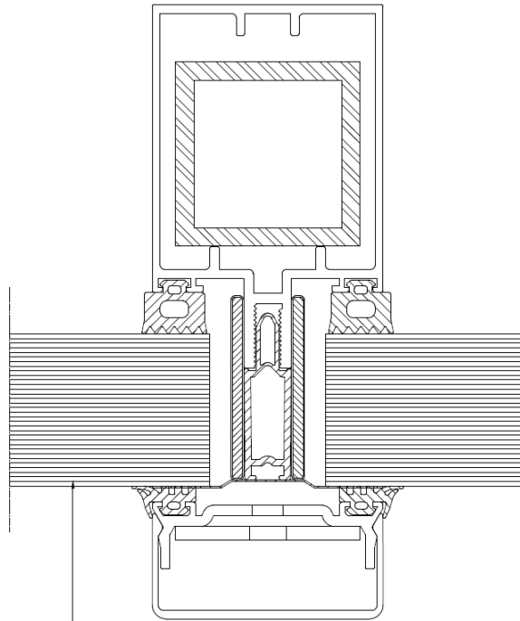
① CONTRAFLAM 60-3 (27 mm thick minimum) (edge-cover 14 mm minimum)
