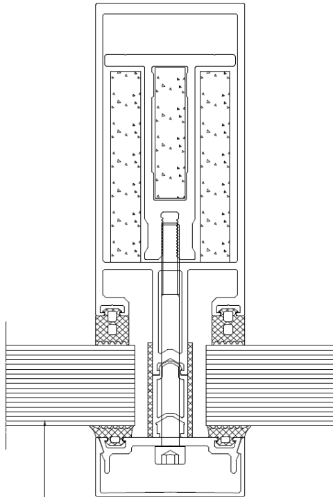
① CONTRAFLAM 60-3 (27 mm thick minimum) (edge-cover 13 mm minimum)
