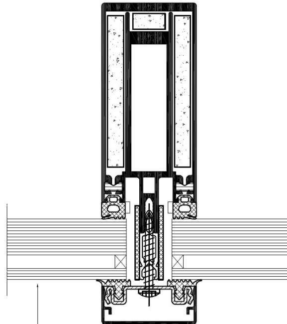
① CONTRAFLAM LITE 30 CLIMAPLUS (edge-cover 13 mm minimum)
